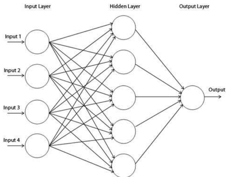
Figure 1. Neural network.
