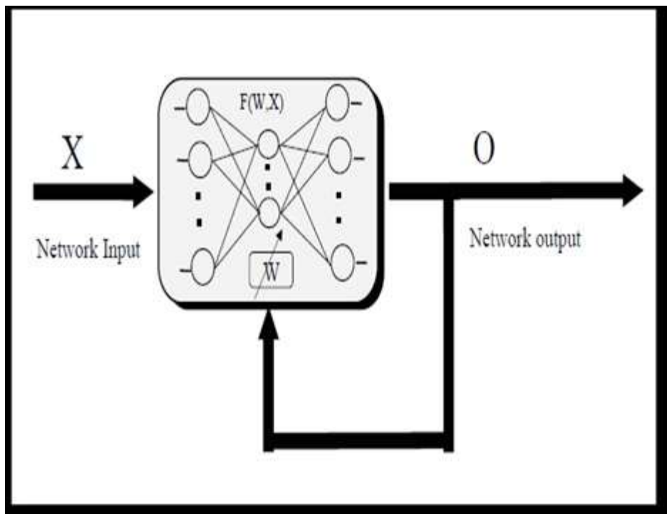
Figure 6. Unsupervised learning.
