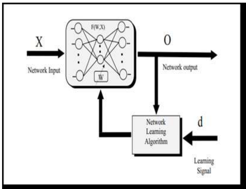
Figure 5. Supervised learning.
